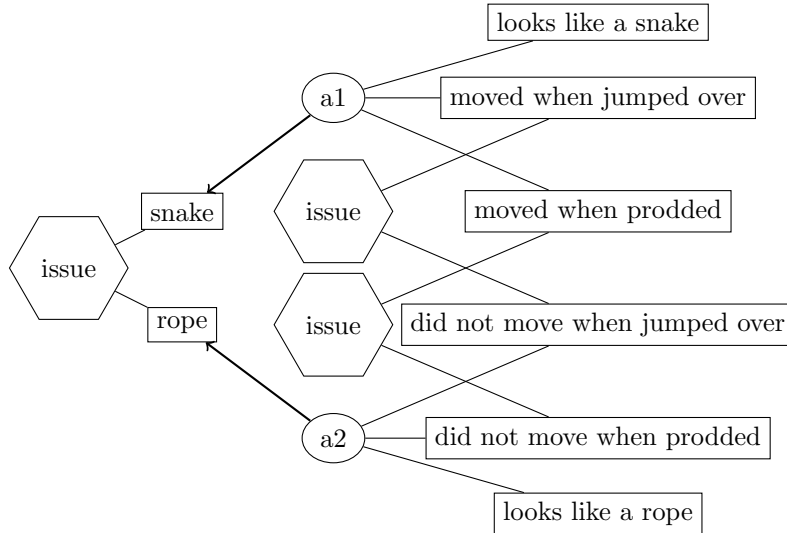
Figure 10. Example Carneades argument graph
