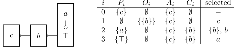
Figure 7. ABA with A = \{b, c\} , \bar{b} = a , \bar{c} = b , and rule a \leftarrow (left); GB-dispute derivation for c (right)
