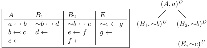
Figure 8. DeLP knowledge base (left) and dialectical tree (right)
