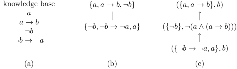
Figure 9. Knowledge base for deductive argumentation (a), inconsistent subsets of that knowledge base (b), and argument tree based on the inconsistent subsets as constructed by compilation-based approach (c)
