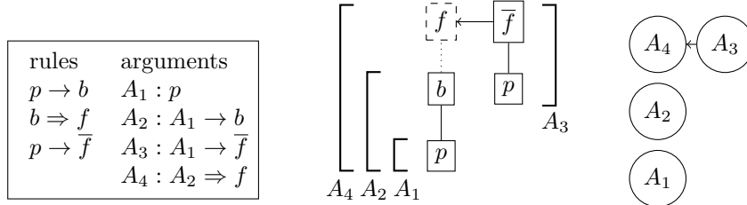
Figure 5. Tweety example knowledge base in ASPIC+ (left) with axiom p , structure of corresponding arguments (middle), and AF (right).
