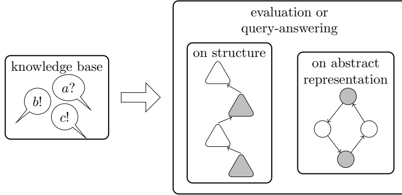
Figure 4. Argumentation process from a computational point of view
