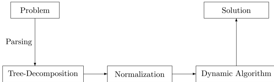
Figure 3. Dynamic-programming approach based on tree-decompositions.
