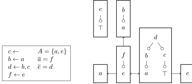
Figure 6. ABA framework (left) and its corresponding arguments and attacks (right)
